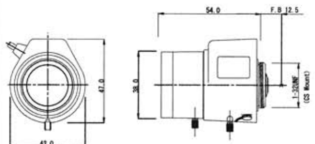
LTV4Z2814GACS
